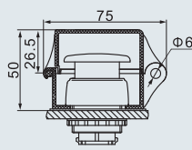
BA8050 Emergency pushbutton with PC protection cover
