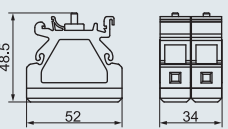
Control button, double (cover mounting)
