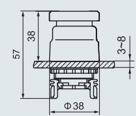
Mushroom turn-to-release emergency control button
